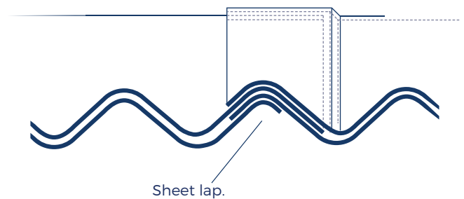
Fig.2 Sheets laid left to right
