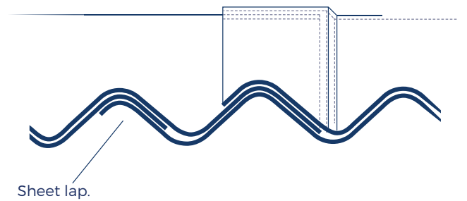
Fig.3 Sheets laid right to left
